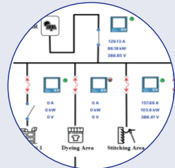
System Architecture (SLD)
